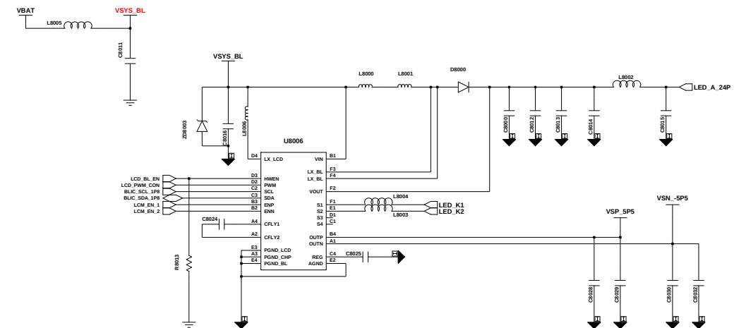
DISPLAY PMIC
